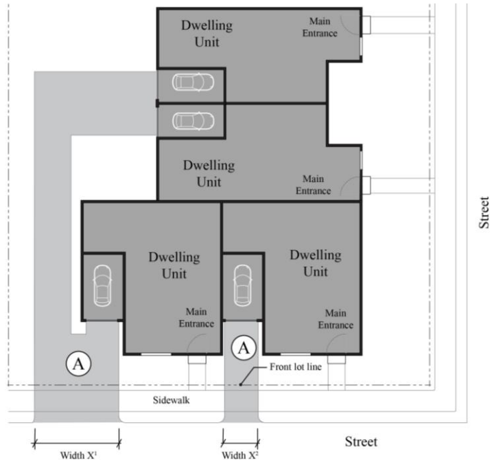
Figure 8.165-4. Triplex and Fourplex: Driveway Approach Options for Multiple Street Frontages
