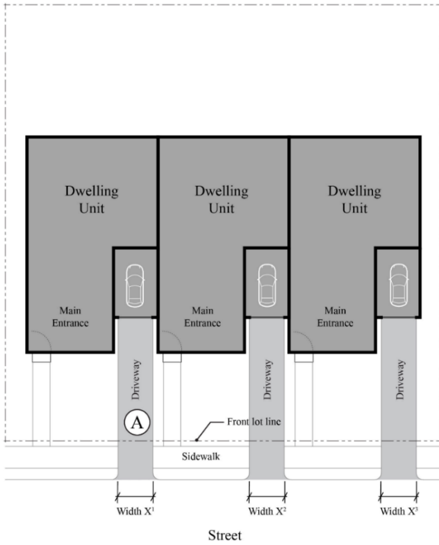
(A) Two driveway approaches not exceeding 40 feet in total width on one frontage (as measured X^1 + X^2 )
